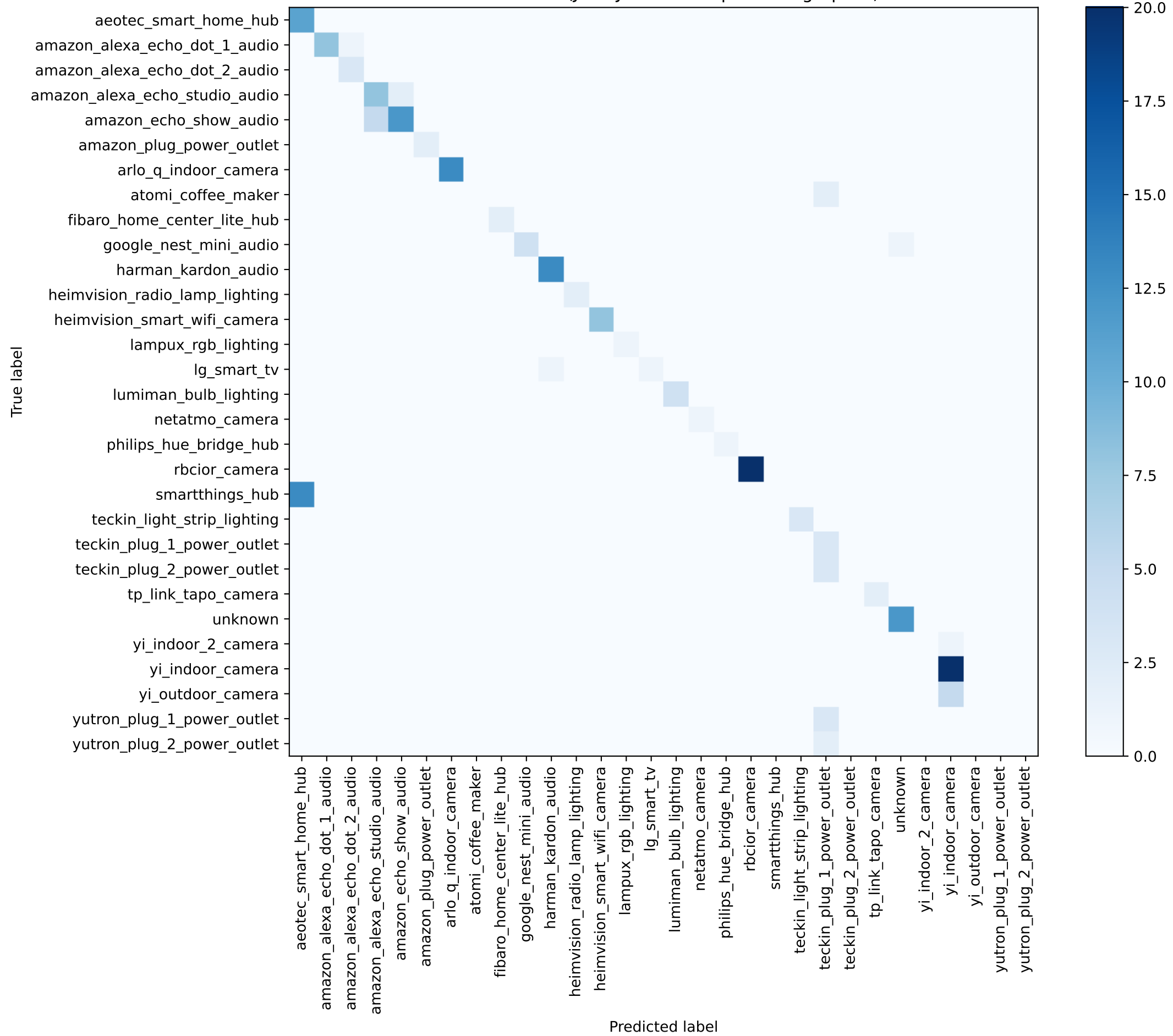
Confusion Matrix - Test (JA4+JA4S decomposed fingerprint) — counts
