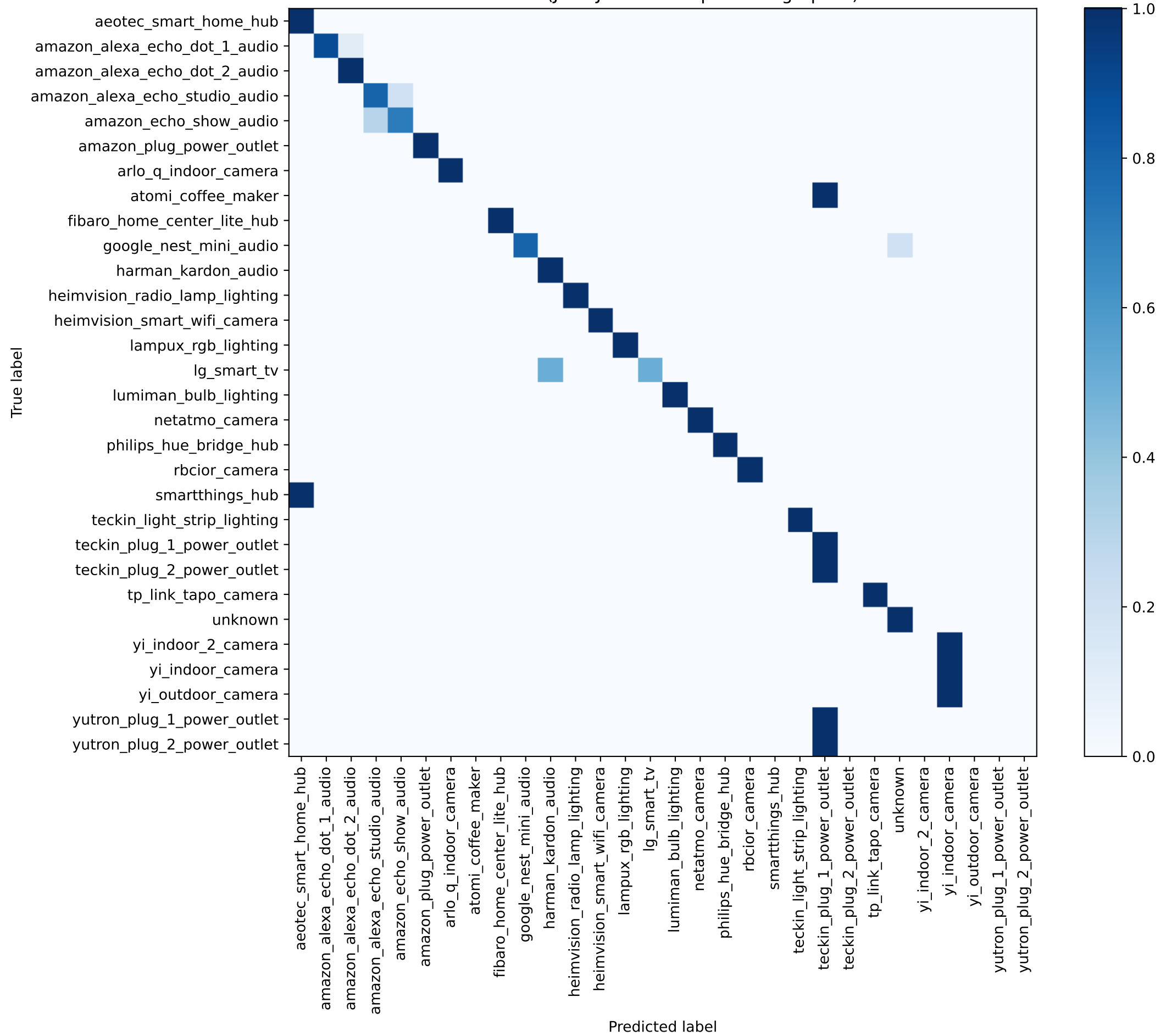
Confusion Matrix - Test (JA4+JA4S decomposed fingerprint) — normalized
