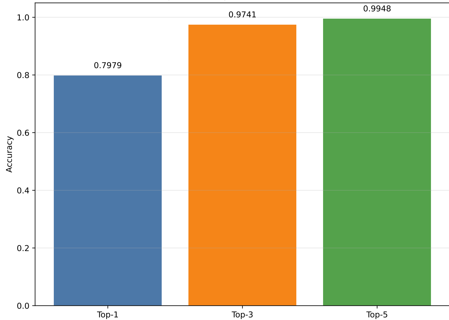
Top-k accuracy (JA4+JA4S features)
