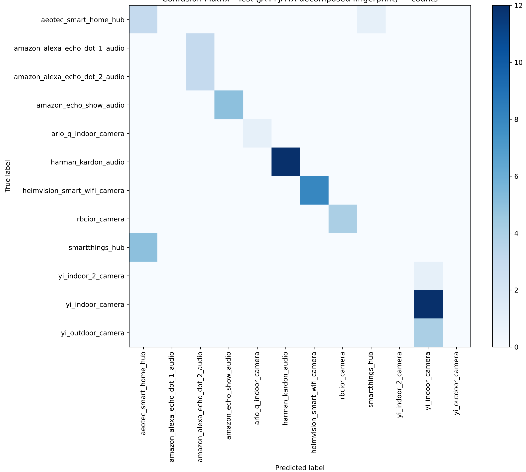
Confusion Matrix - Test (JA4+JA4X decomposed fingerprint) — counts
