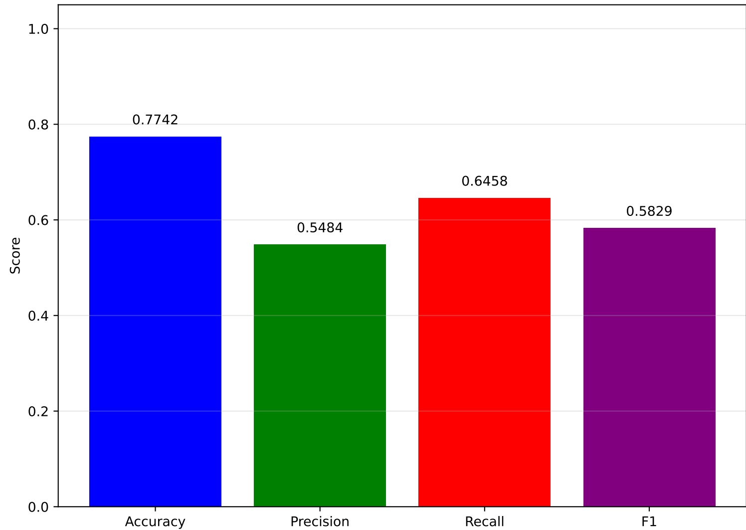
Test Metrics (JA4 + JA4X features)
