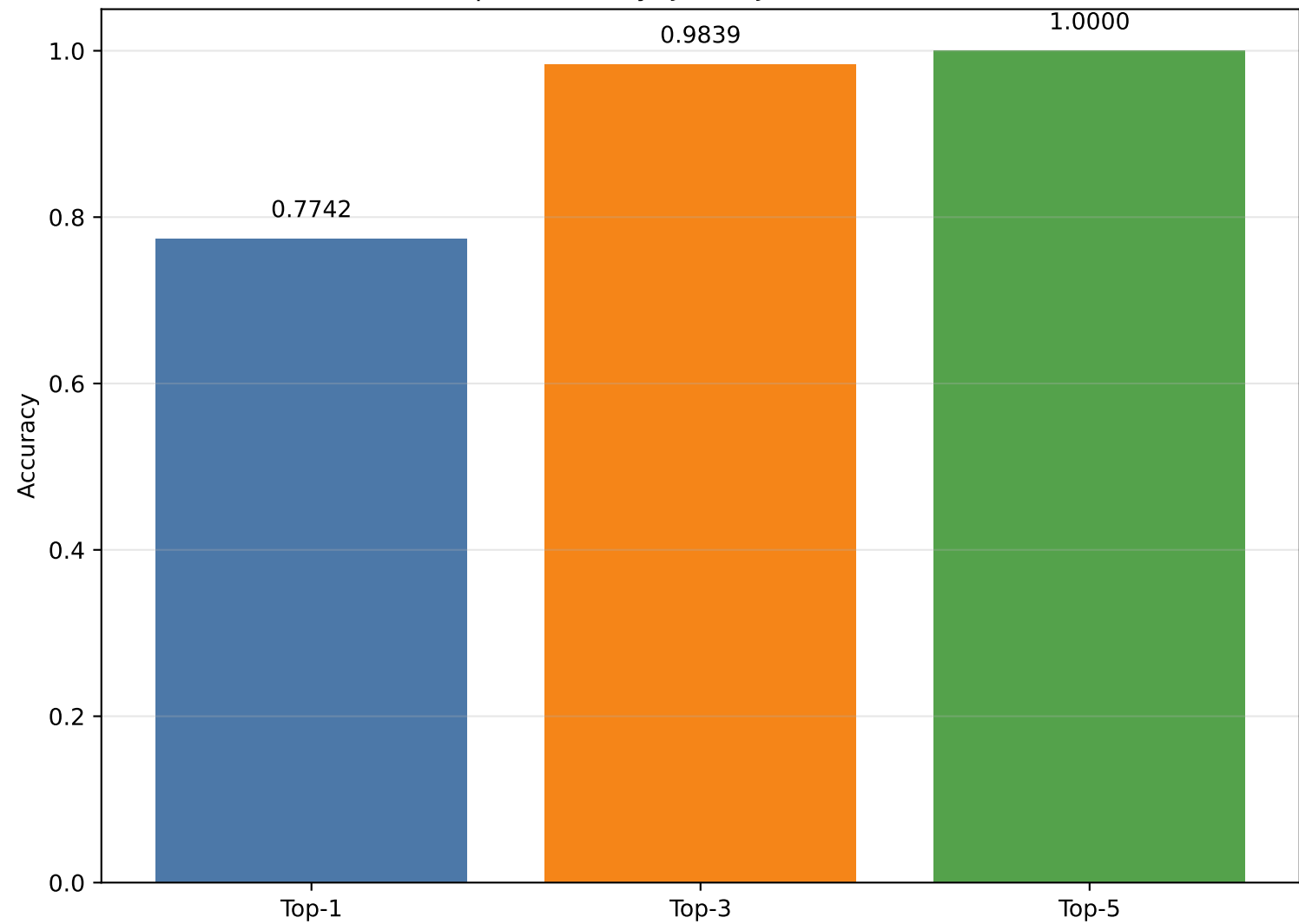
Top-k accuracy (JA4 + JA4X features)
