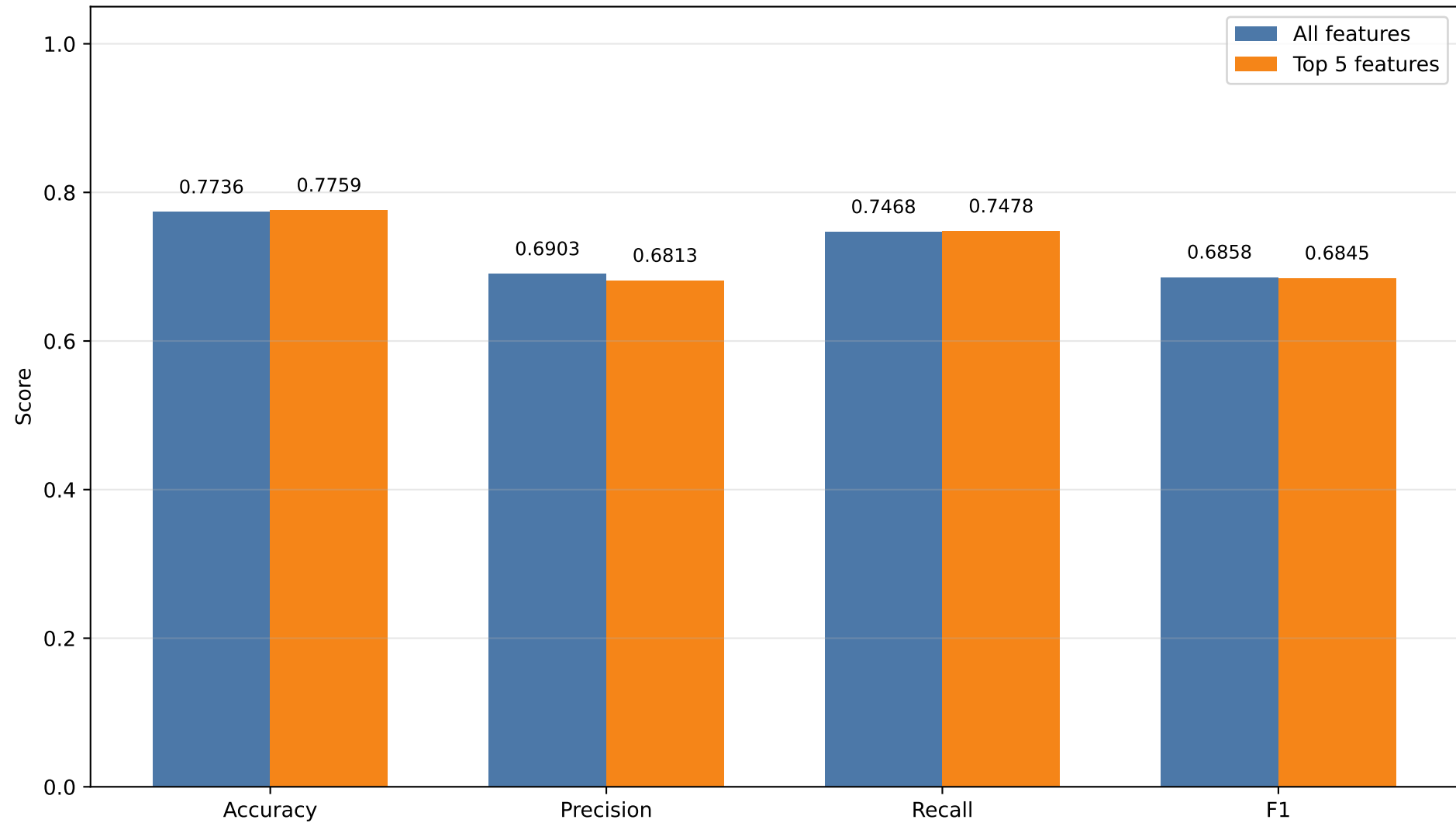
JA4 features vs Top 5 features - Test Metrics
