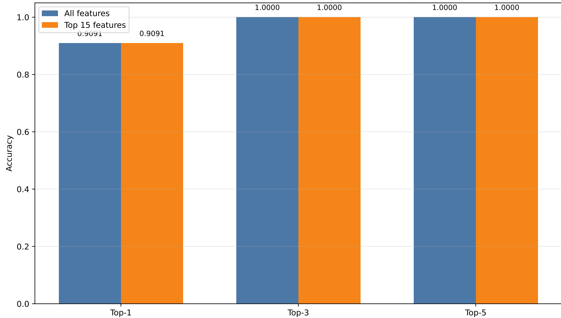
JA4+ features vs Top 15 features - Top-k accuracy
