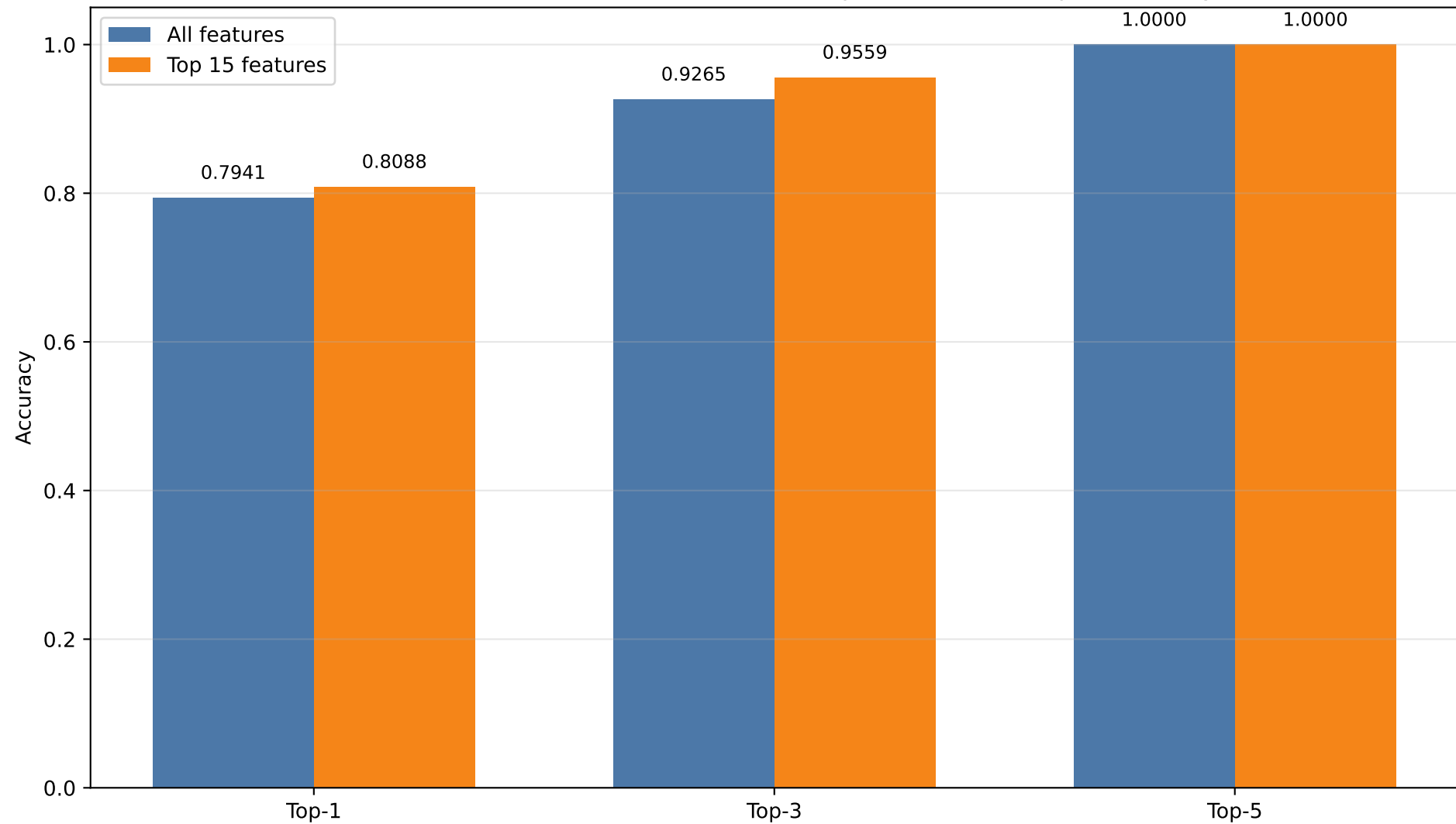
JA4 + JA4S + JA4T + JA4TS features vs Top 15 features - Top-k accuracy
