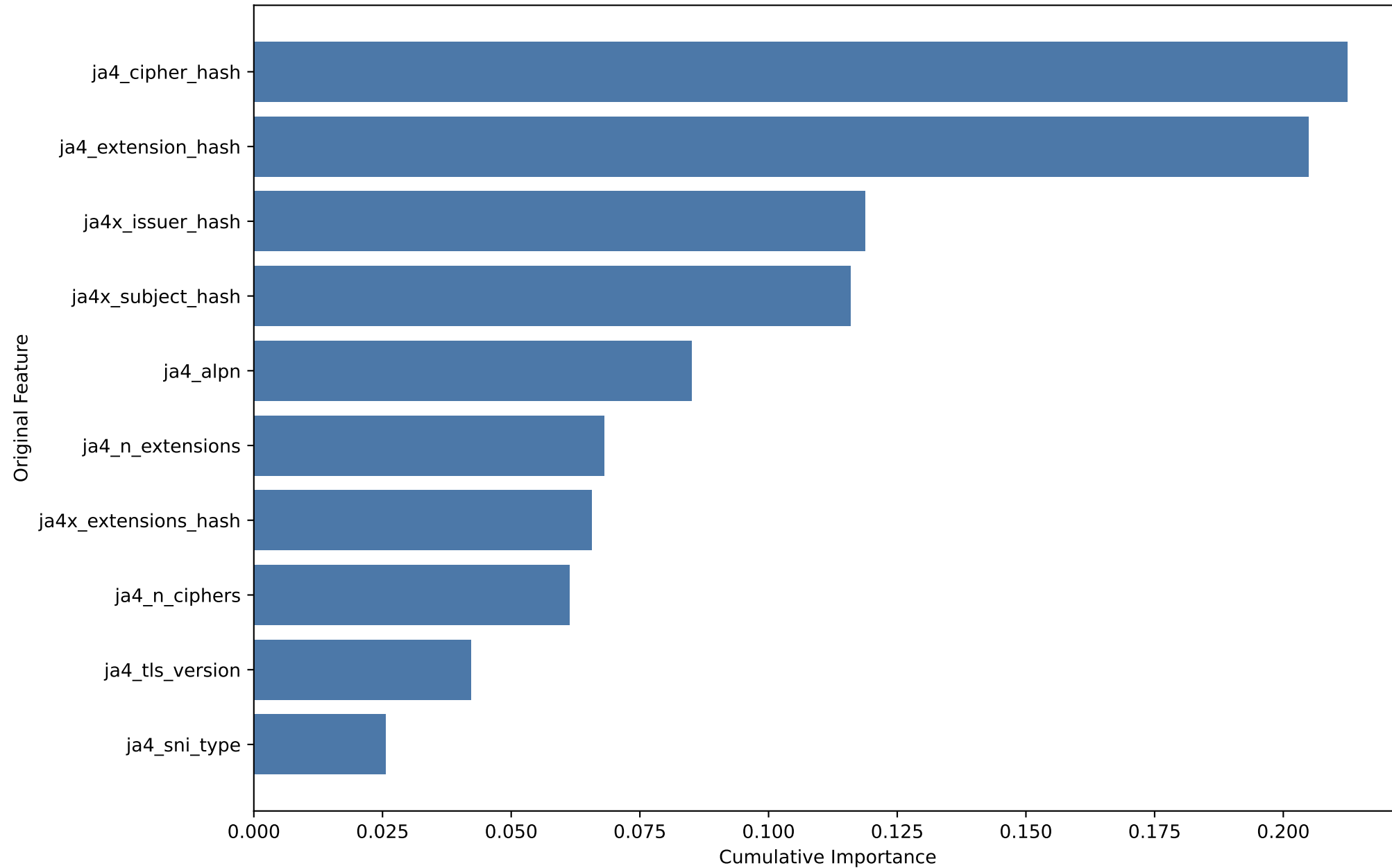
Top 10 Most Important Original Features
