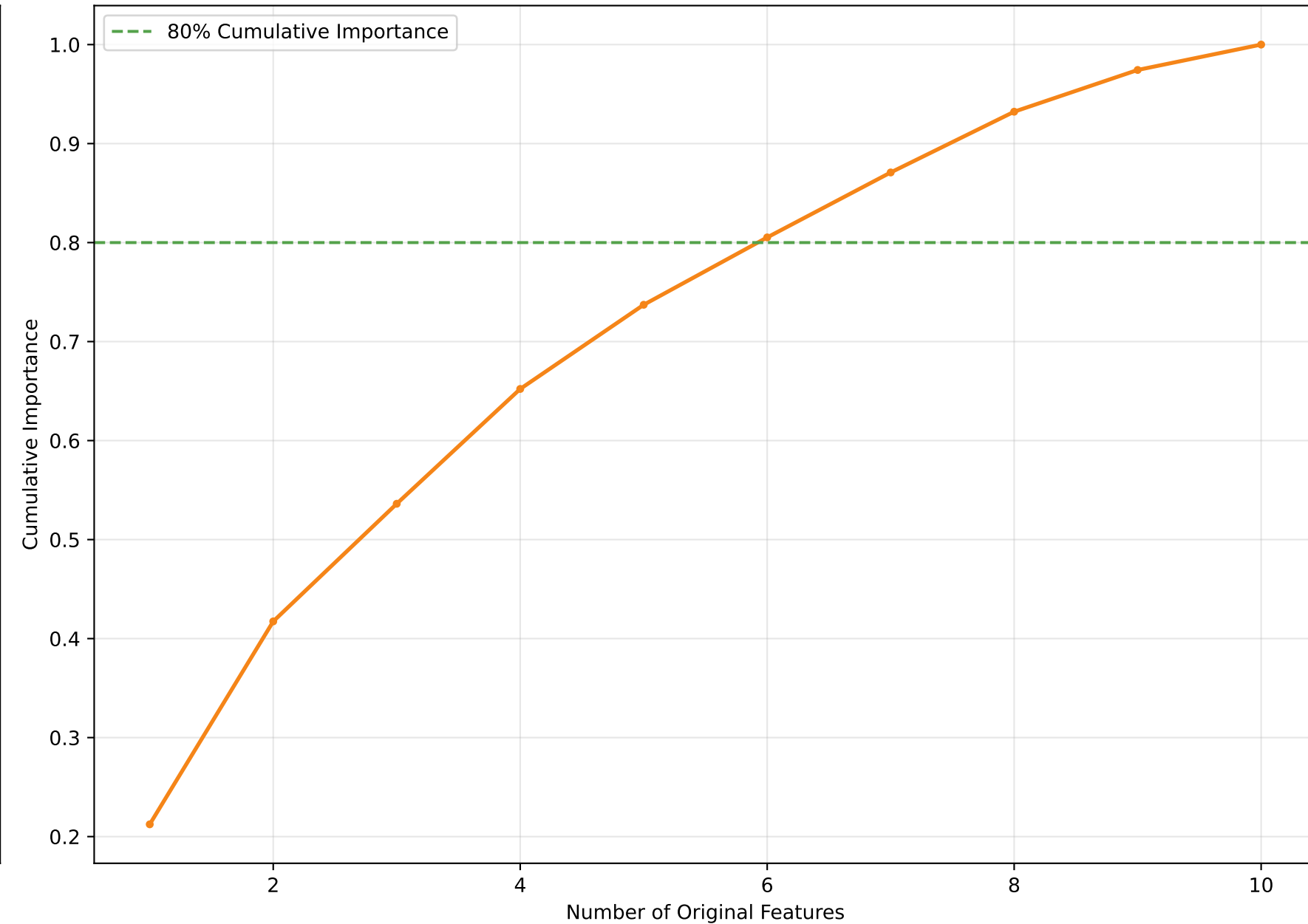
Cumulative Importance by Original Feature
