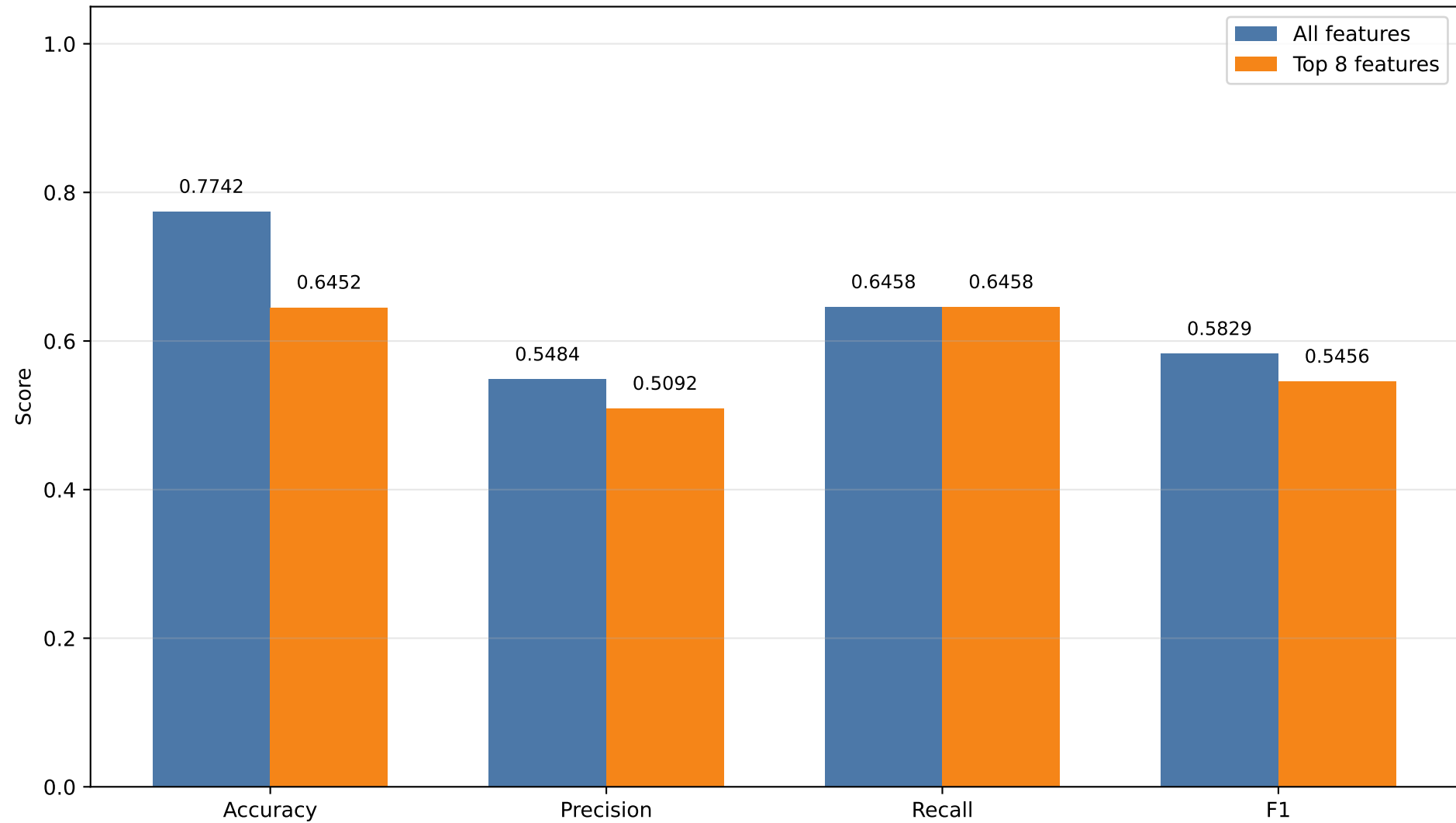
JA4 + JA4X features vs Top 8 features - Test Metrics
