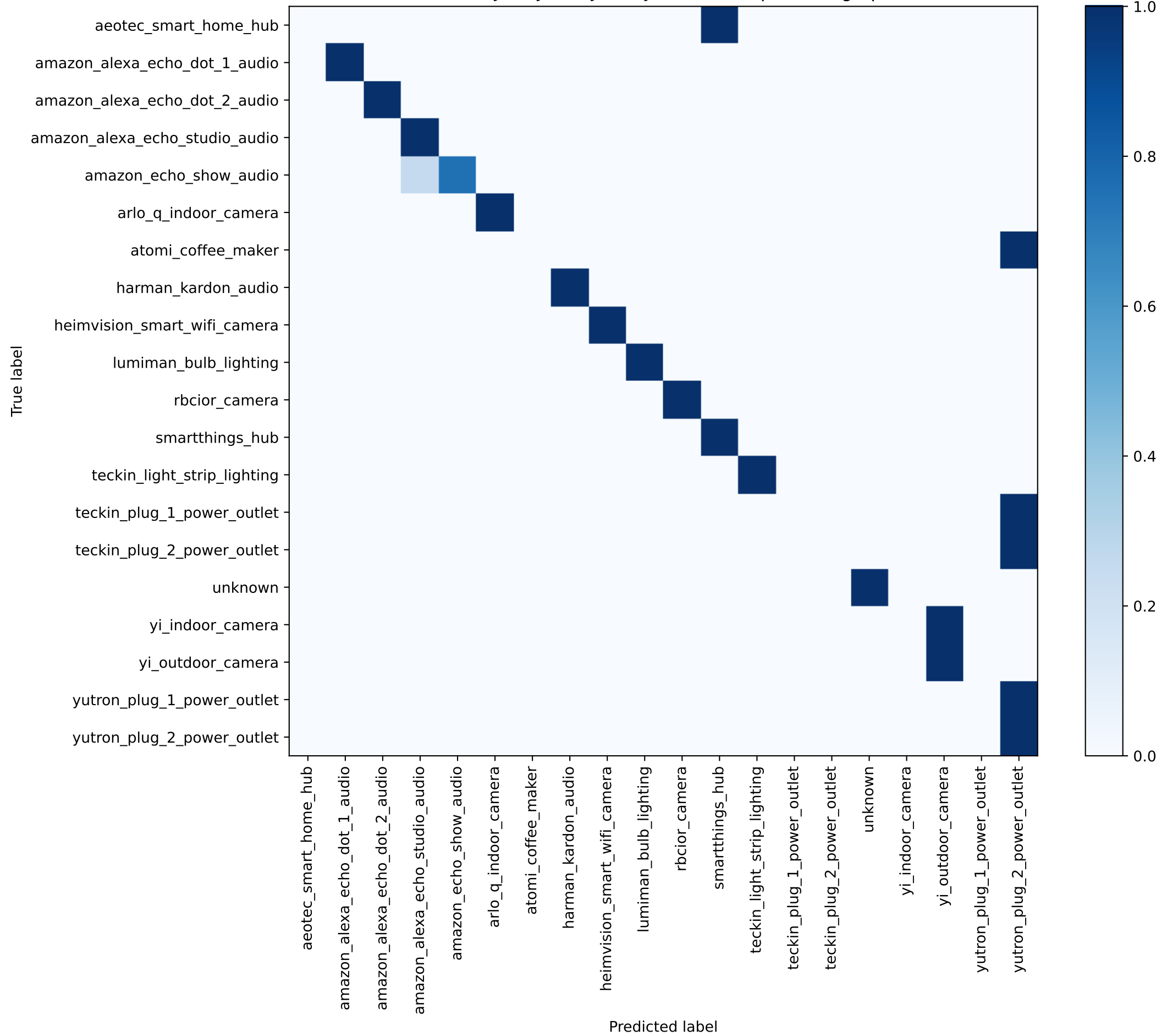
Confusion Matrix - Test (JA4+JA4S+JA4T+JA4TS decomposed fingerprint) — normalized
