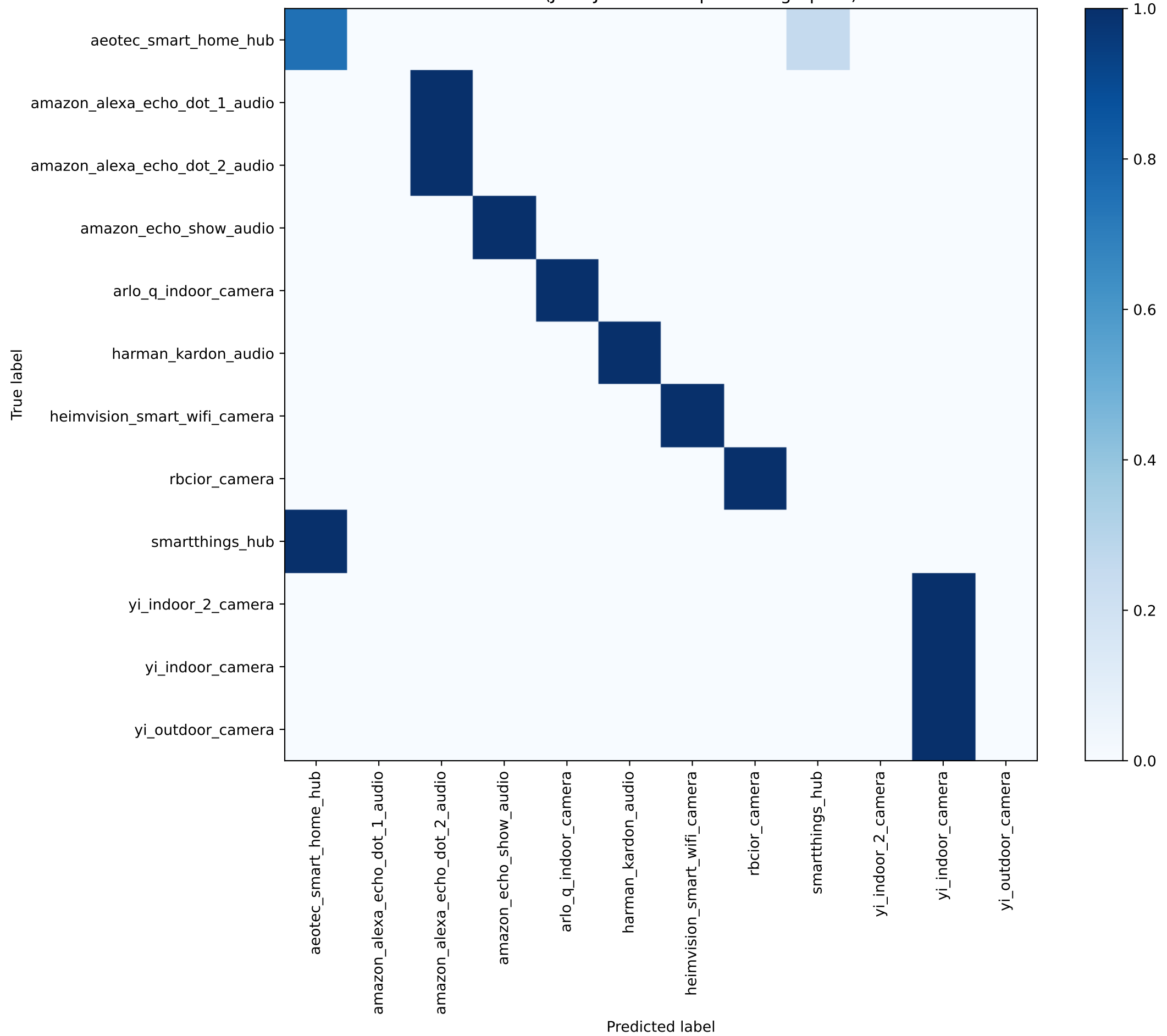
Confusion Matrix - Test (JA4+JA4X decomposed fingerprint) — normalized
