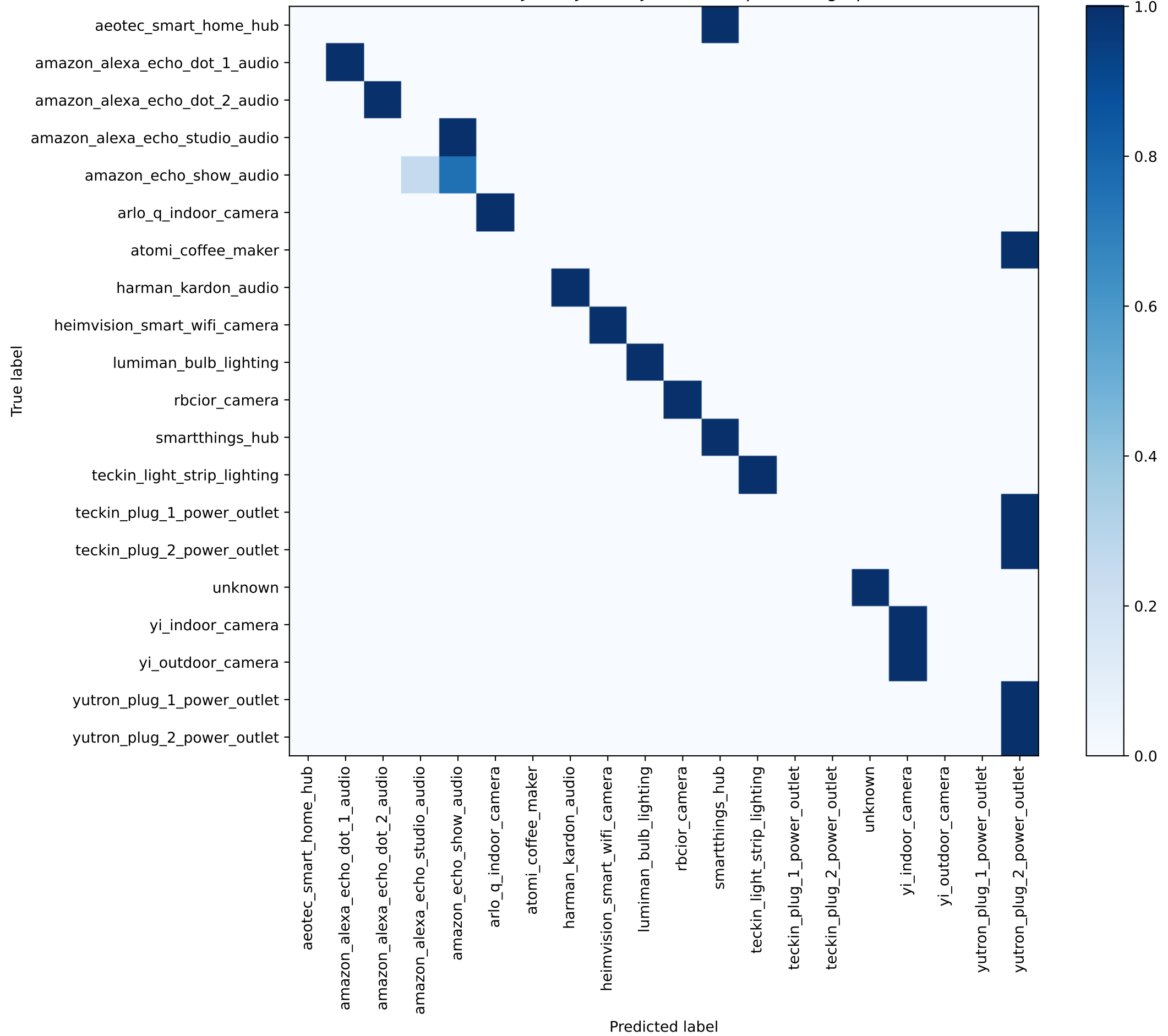
Confusion Matrix - Test (JA4 + JA4S + JA4T decomposed fingerprint) - normalized
