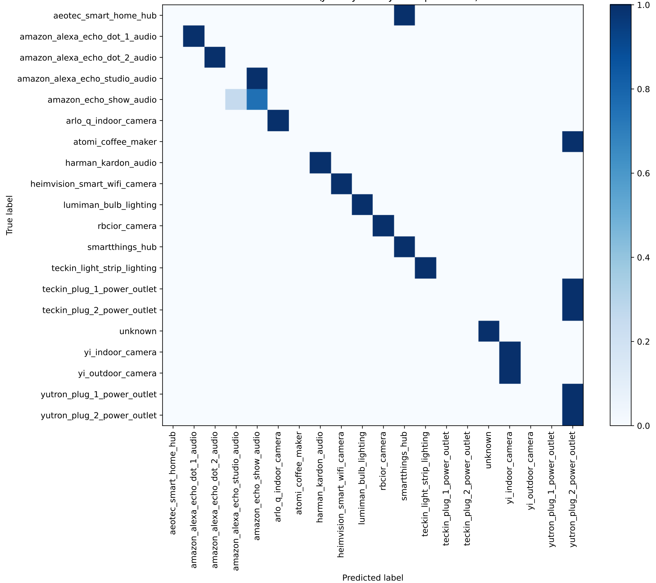
Confusion Matrix - Test (JA4 + JA4S + JA4T top features) - normalized
