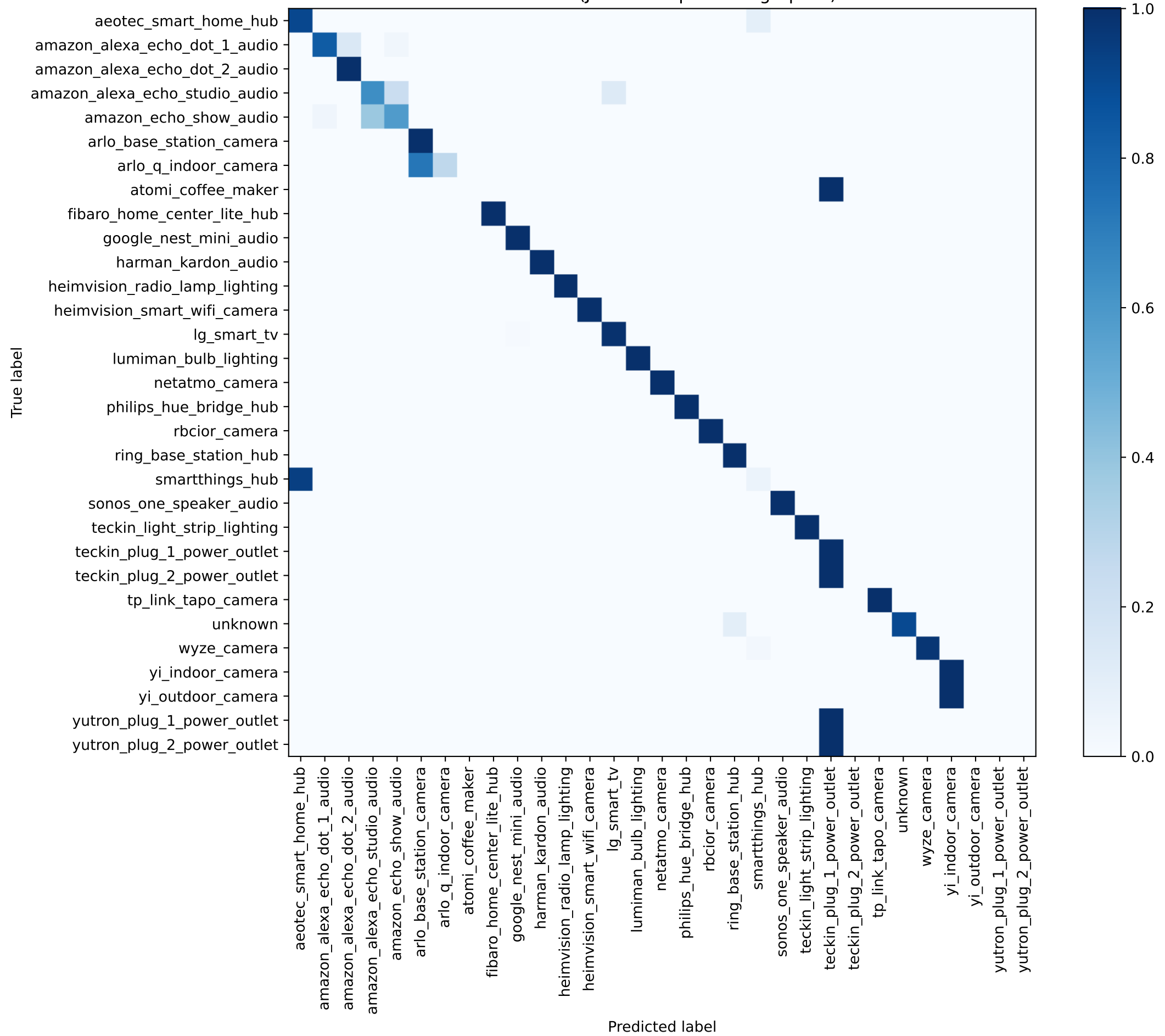
Confusion Matrix - Test (JA4 decomposed fingerprint) - normalized
