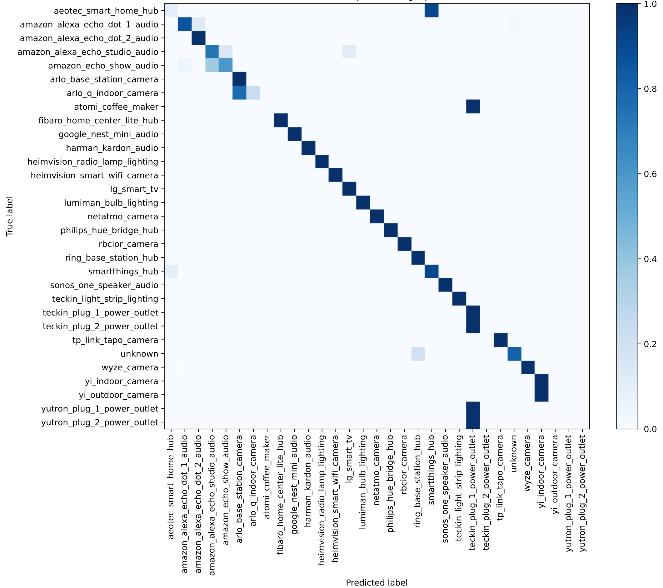
Confusion Matrix - Test (JA4 full fingerprint) - normalized
