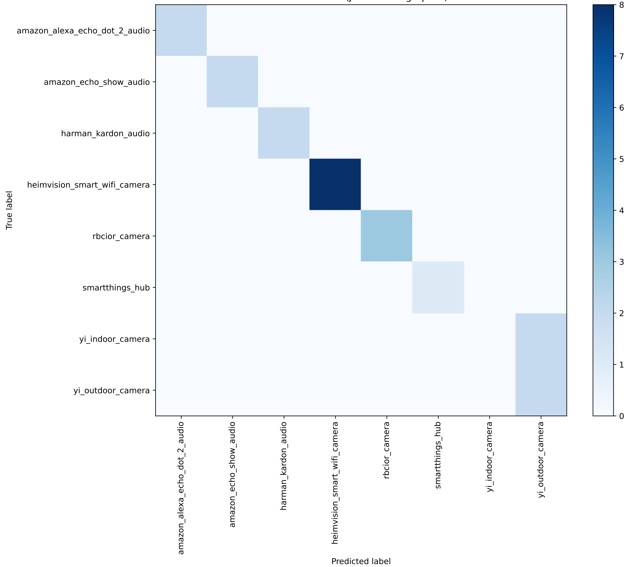
Confusion Matrix - Test (JA4+ full fingerprint) - counts
