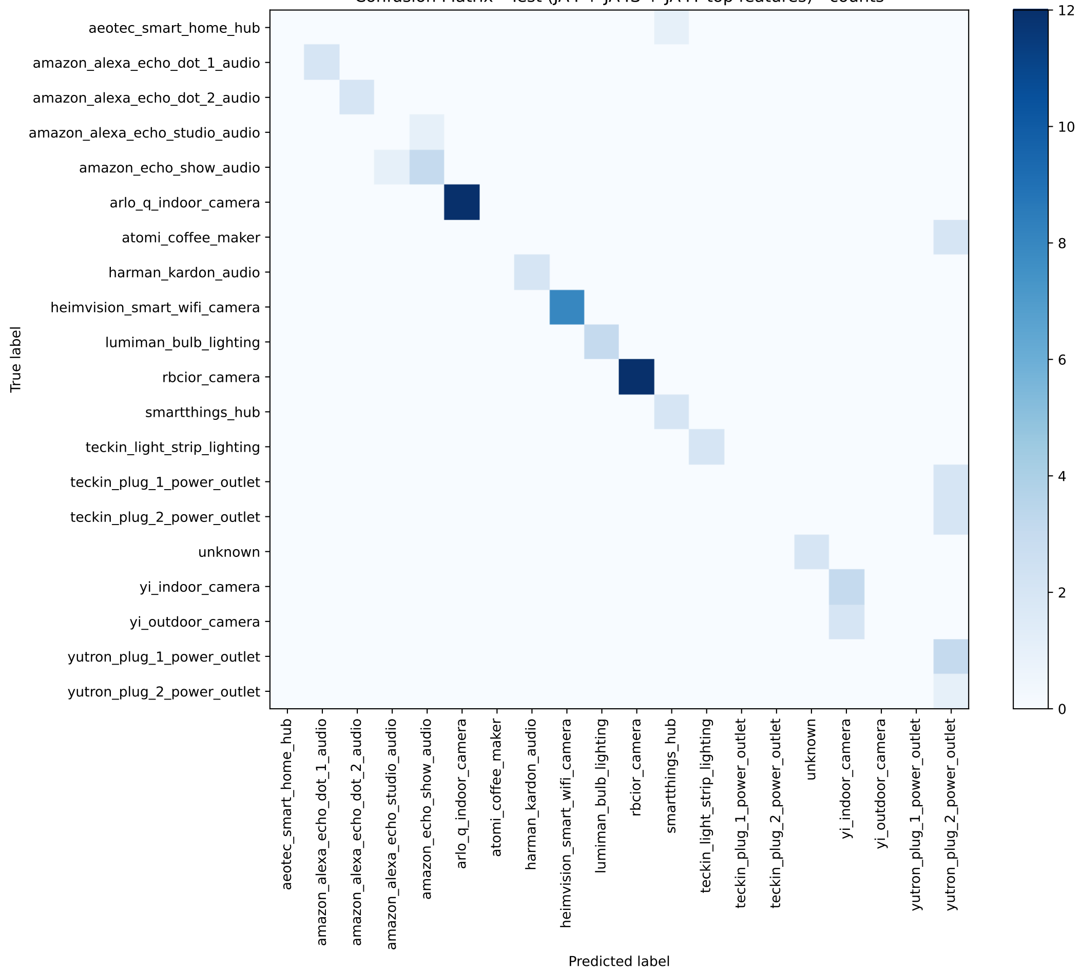
Confusion Matrix - Test (JA4 + JA4S + JA4T top features) - counts
