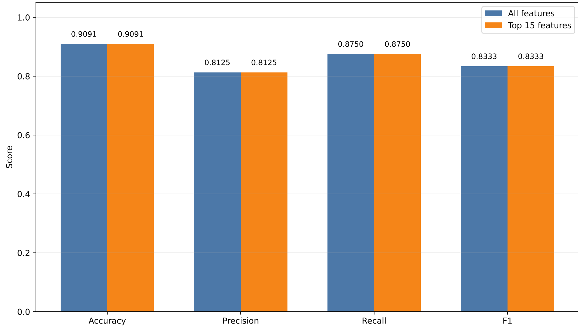
JA4+ features vs Top 15 features - Test Metrics
