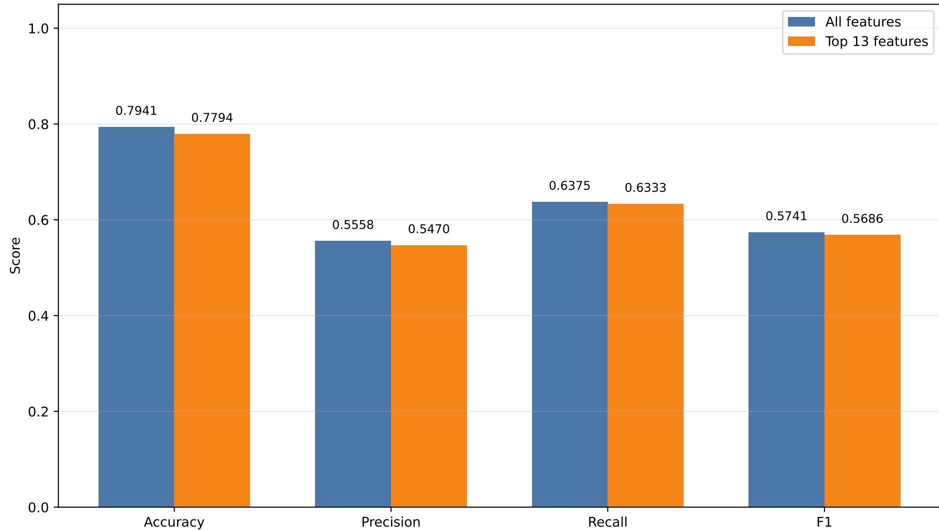
JA4 + JA4S + JA4TS features vs Top 13 features - Test Metrics
