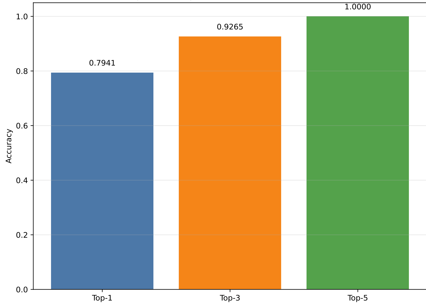
Top-k accuracy (JA4 + JA4S + JA4TS features)
