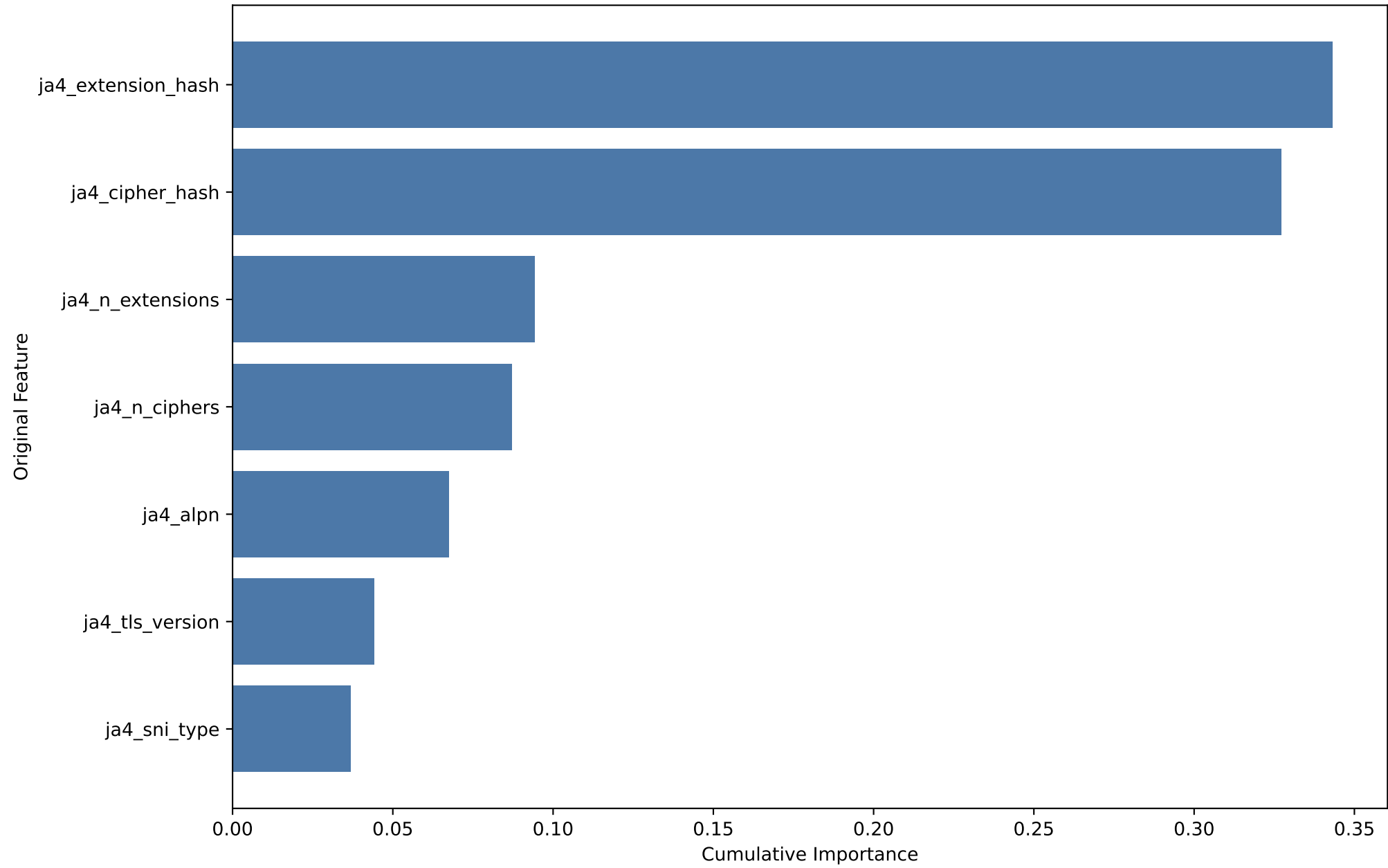
Top 7 Most Important Original Features
