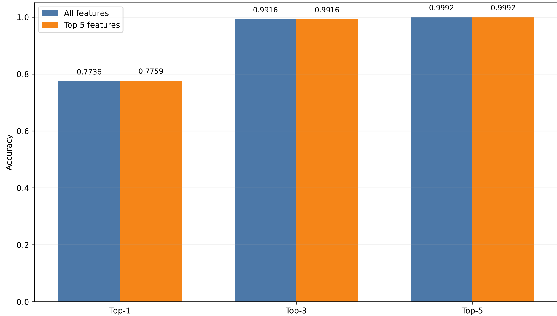
JA4 features vs Top 5 features - Top-k accuracy
