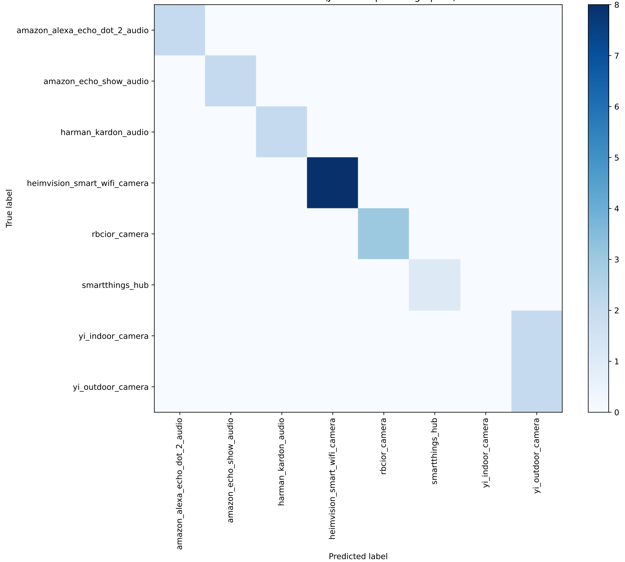
Confusion Matrix - Test (JA4+ complete fingerprint) — counts
