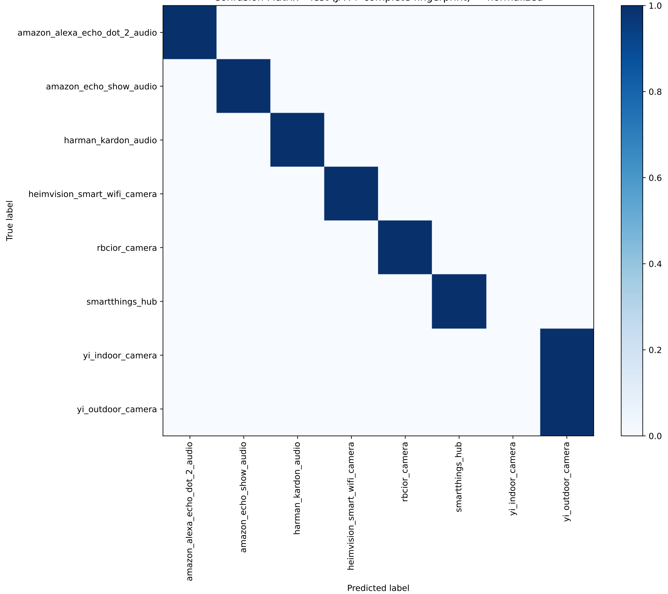
Confusion Matrix - Test (JA4+ complete fingerprint) — normalized
