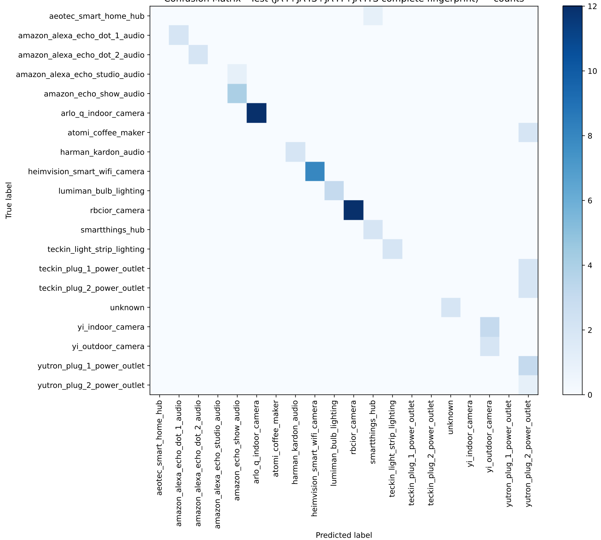
Confusion Matrix - Test (JA4+JA4S+JA4T+JA4TS complete fingerprint) — counts
