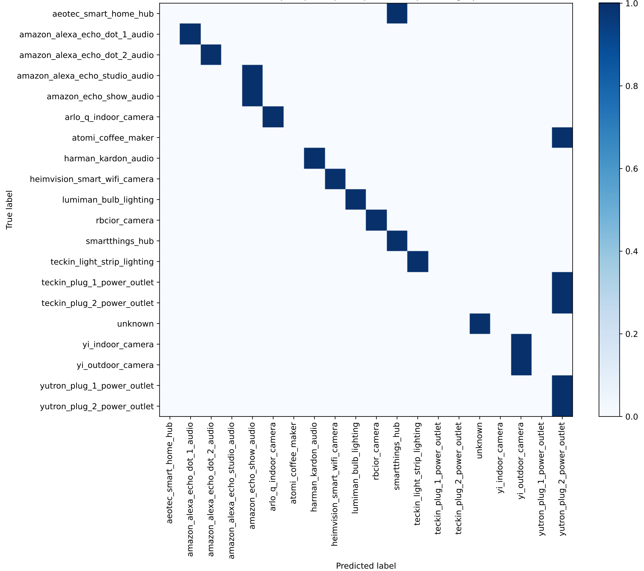
Confusion Matrix - Test (JA4+JA4S+JA4T+JA4TS complete fingerprint) — normalized
