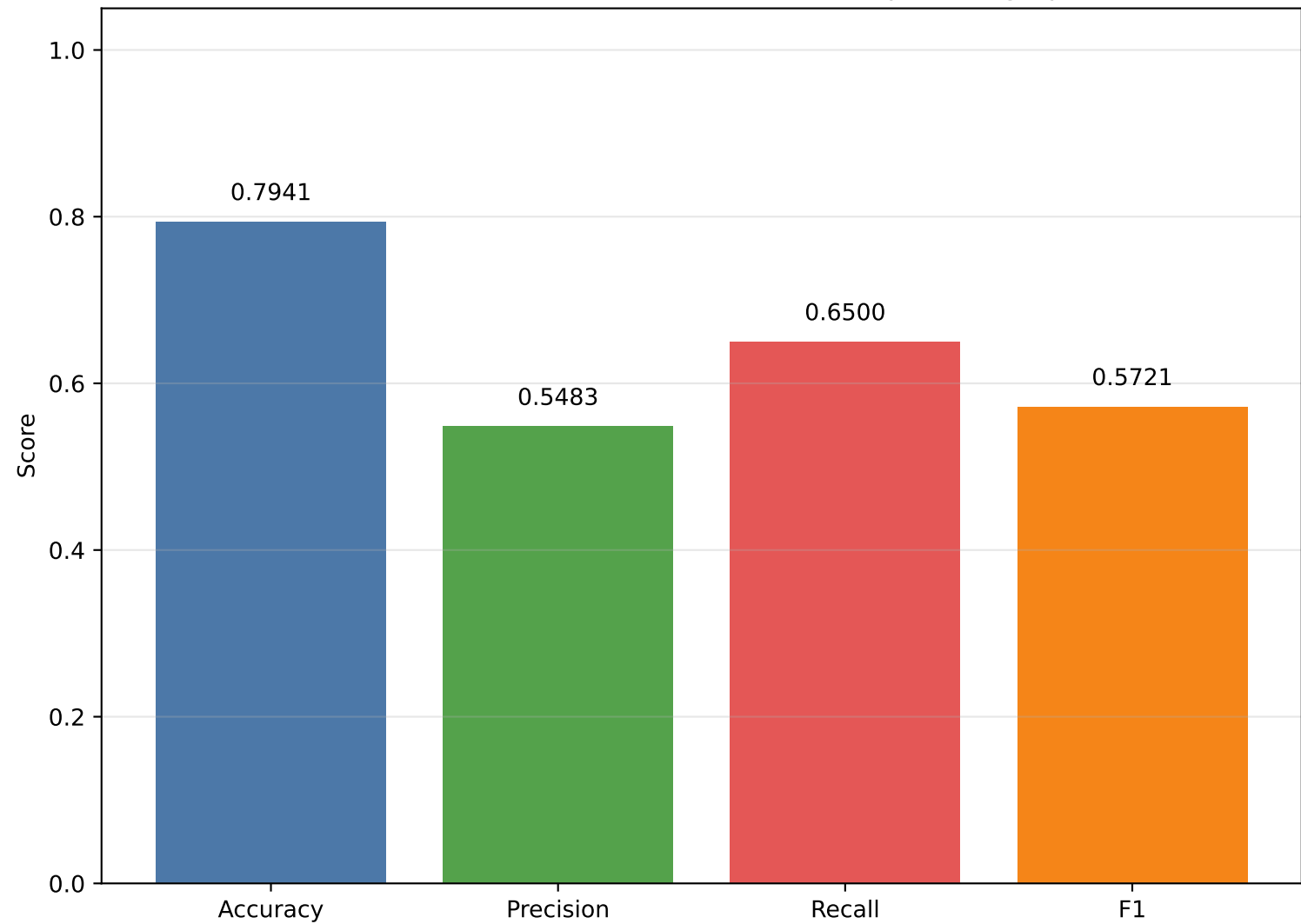
Test Metrics (JA4 + JA4S + JA4T + JA4TS complete fingerprints)
