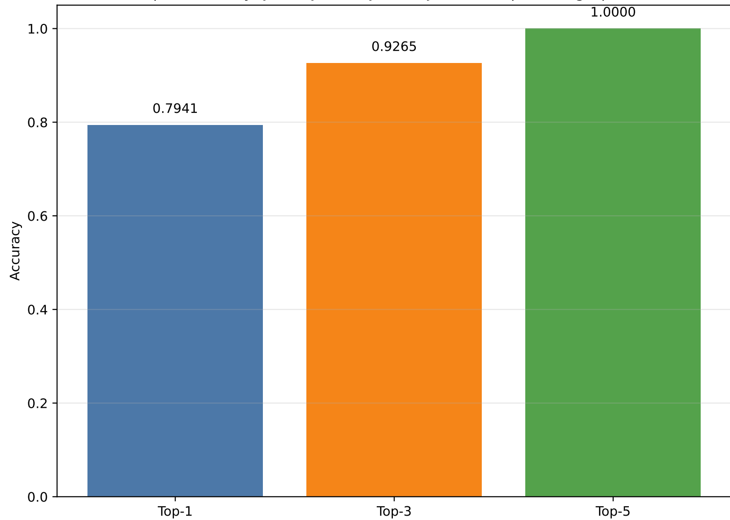
Top-k accuracy (JA4 + JA4S + JA4T + JA4TS complete fingerprints)
