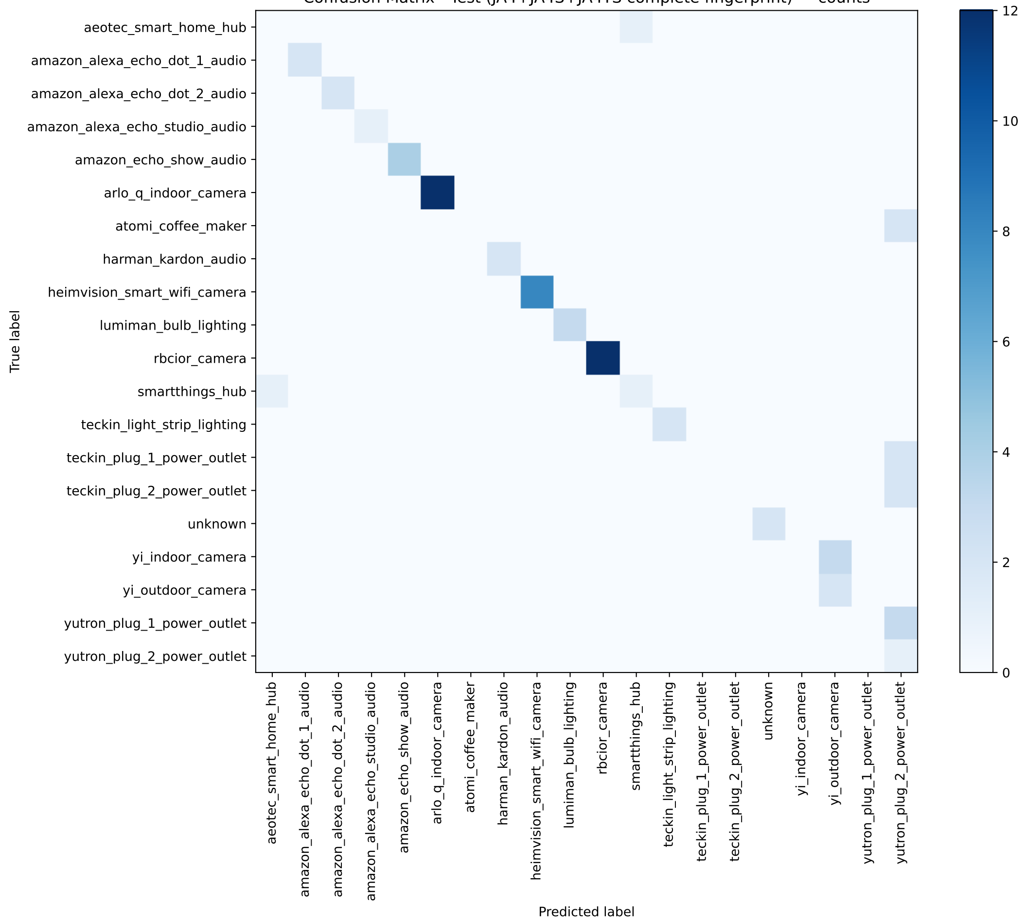
Confusion Matrix - Test (JA4+JA4S+JA4TS complete fingerprint) — counts
