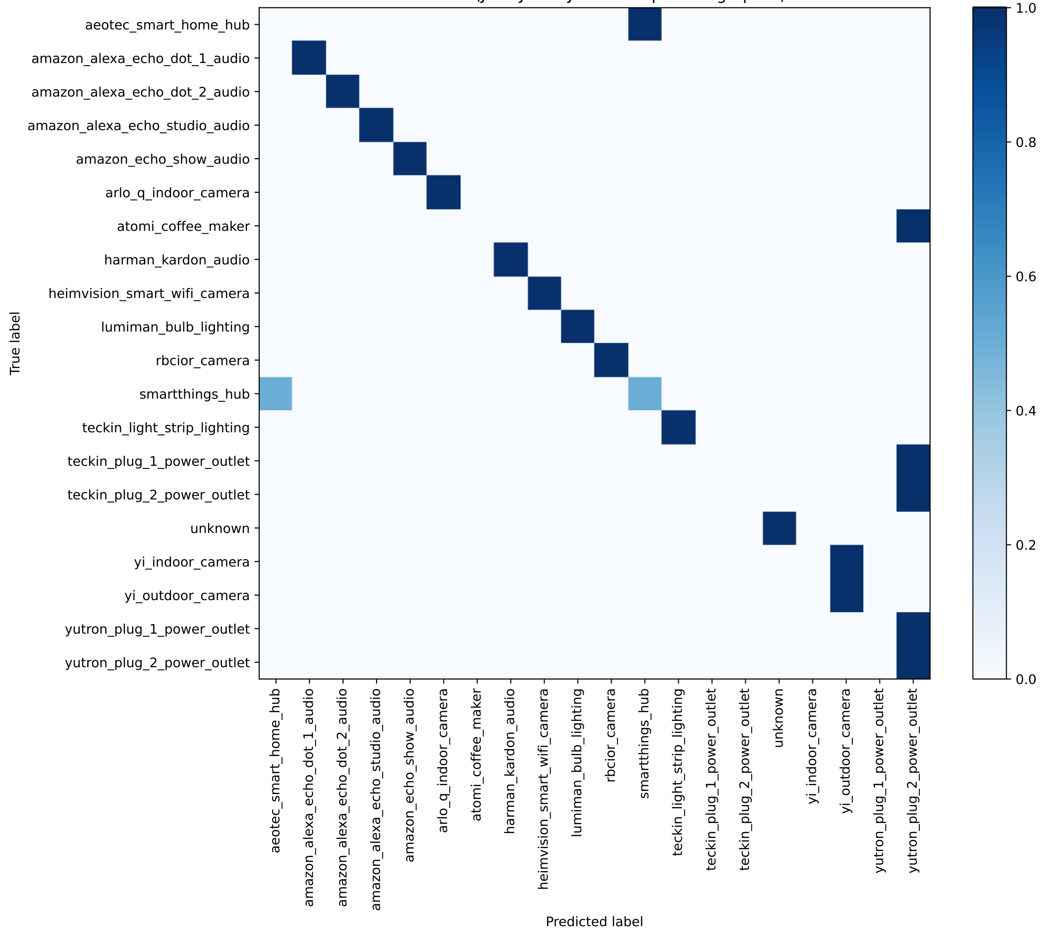
Confusion Matrix - Test (JA4+JA4S+JA4TS complete fingerprint) — normalized
