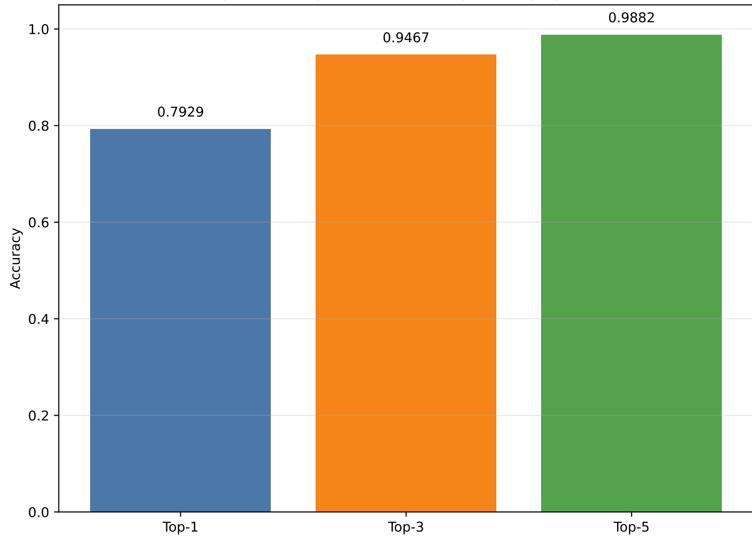
Top-k accuracy (JA4 + JA4S complete fingerprints)
