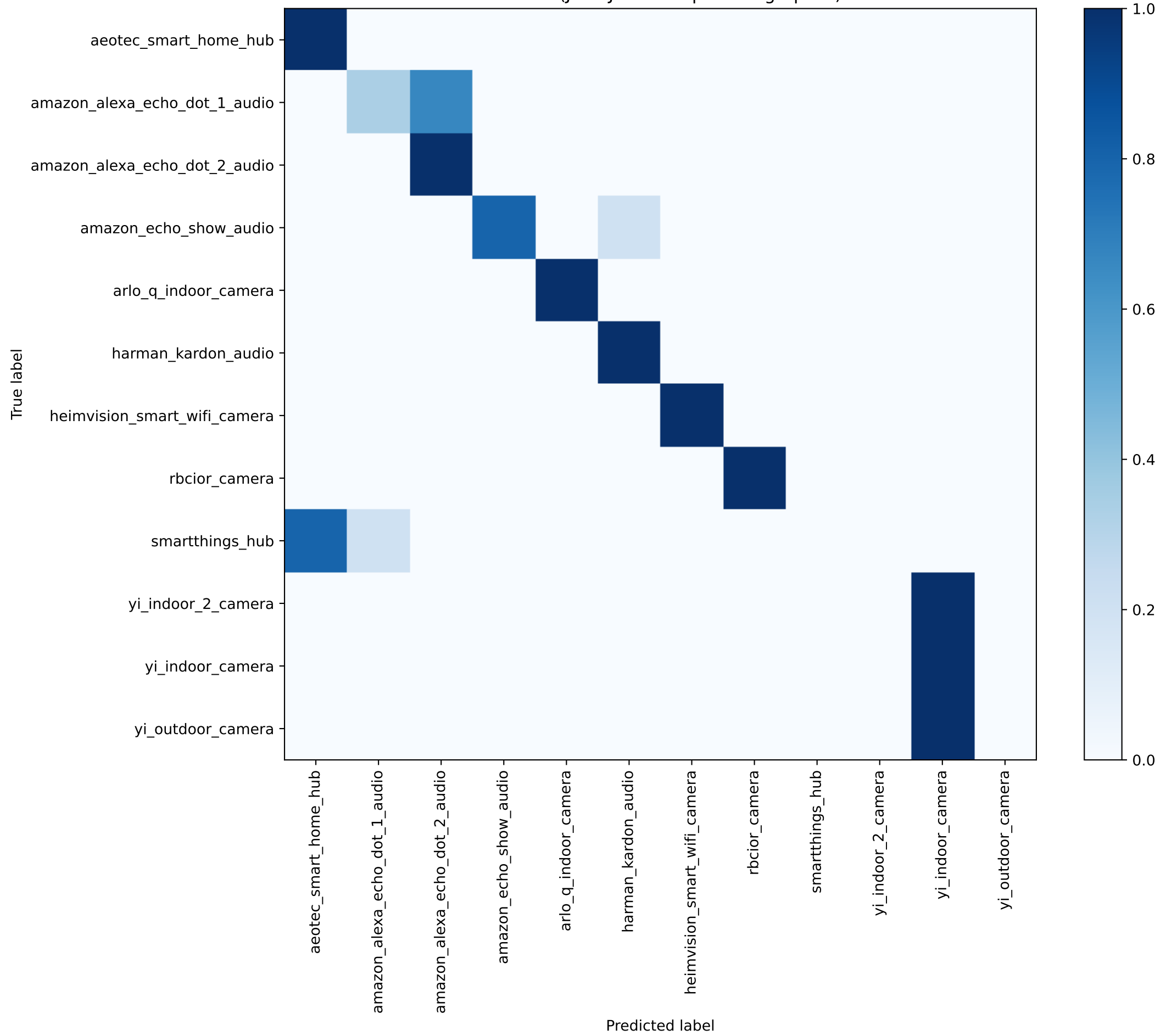
Confusion Matrix - Test (JA4+JA4X complete fingerprint) — normalized
