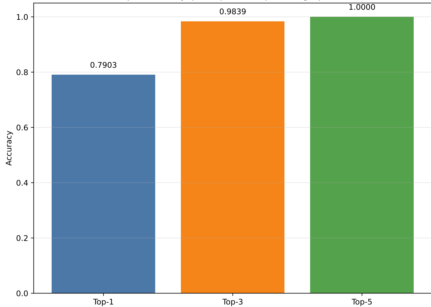
Top-k accuracy (JA4 + JA4X complete fingerprints)
