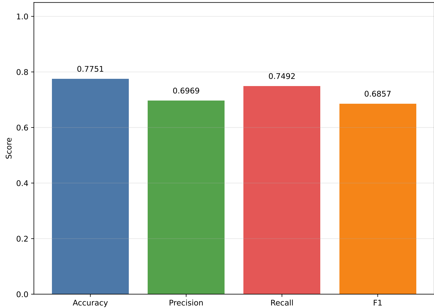
Test Metrics (JA4 full fingerprint)
