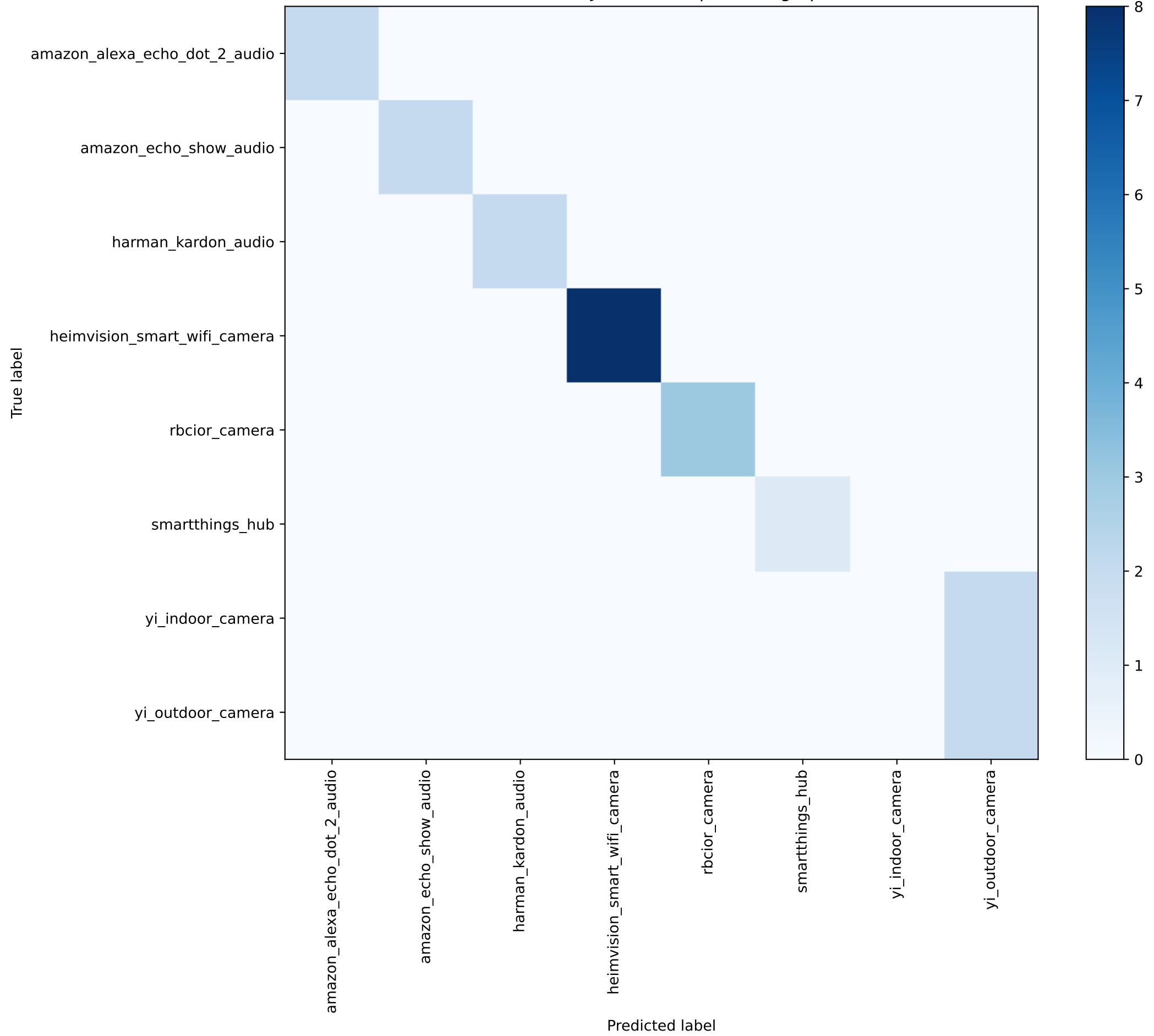
Confusion Matrix - Test (JA4+ decomposed fingerprint) — counts
