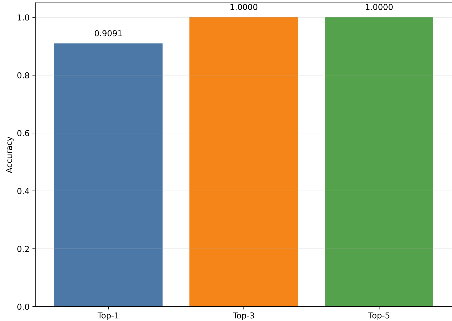
Top-k accuracy (JA4+ complete fingerprints)
