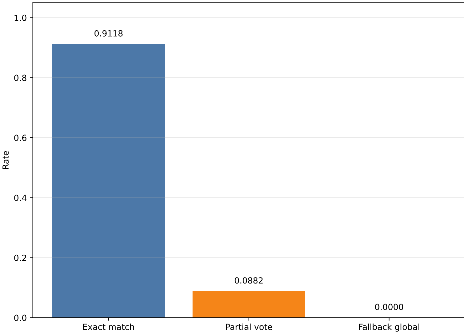
Dictionary Usage Breakdown (JA4 + JA4S + JA4T + JA4TS complete fingerprints)
