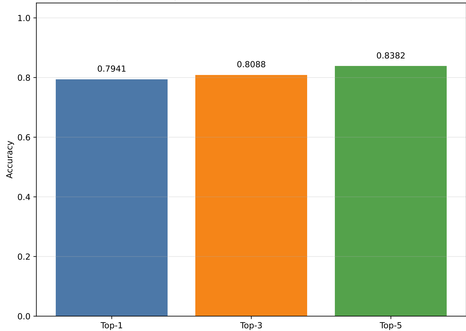
Top-k accuracy (JA4 + JA4S + JA4TS complete fingerprints)
