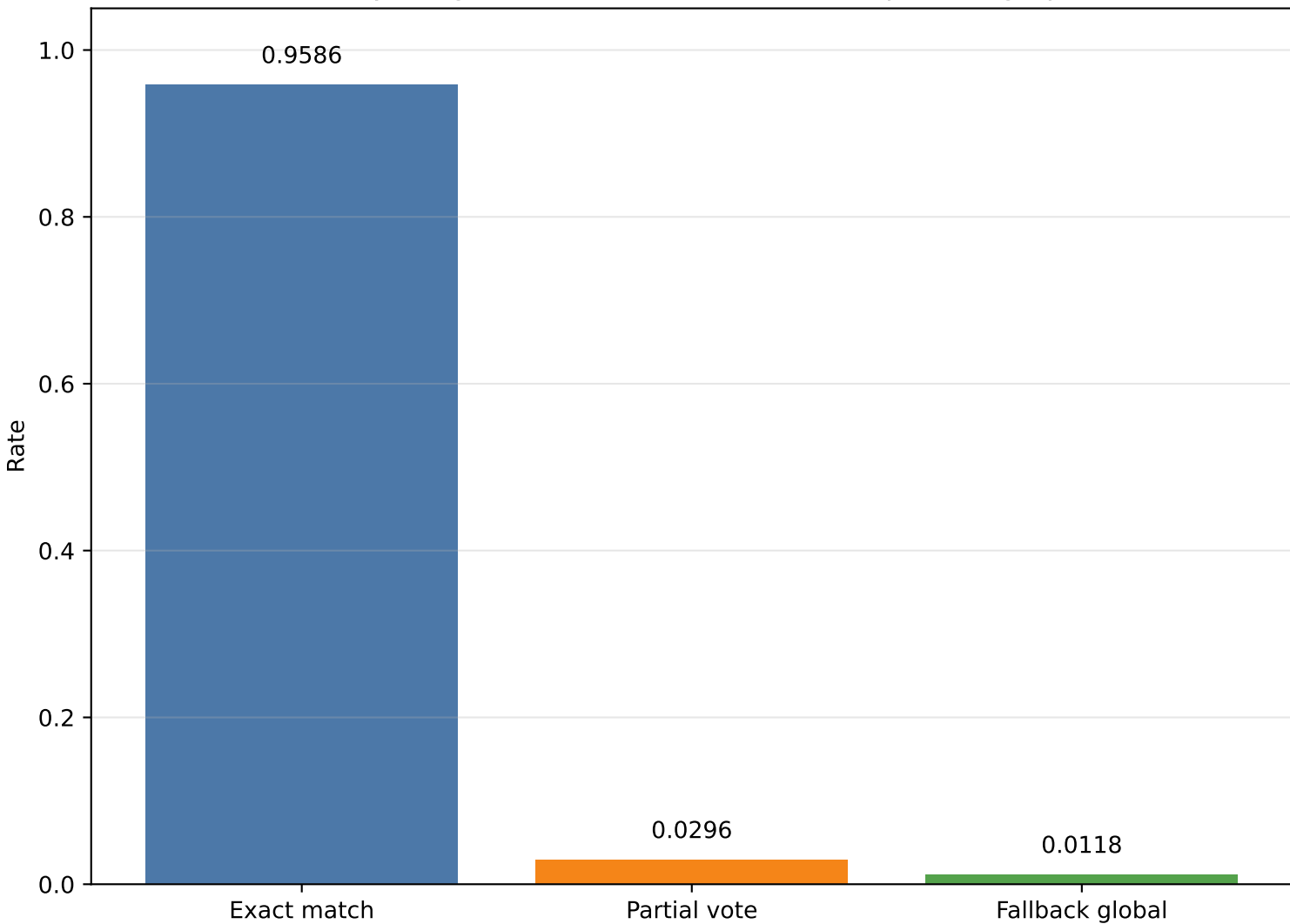
Dictionary Usage Breakdown (JA4 + JA4S complete fingerprints)
