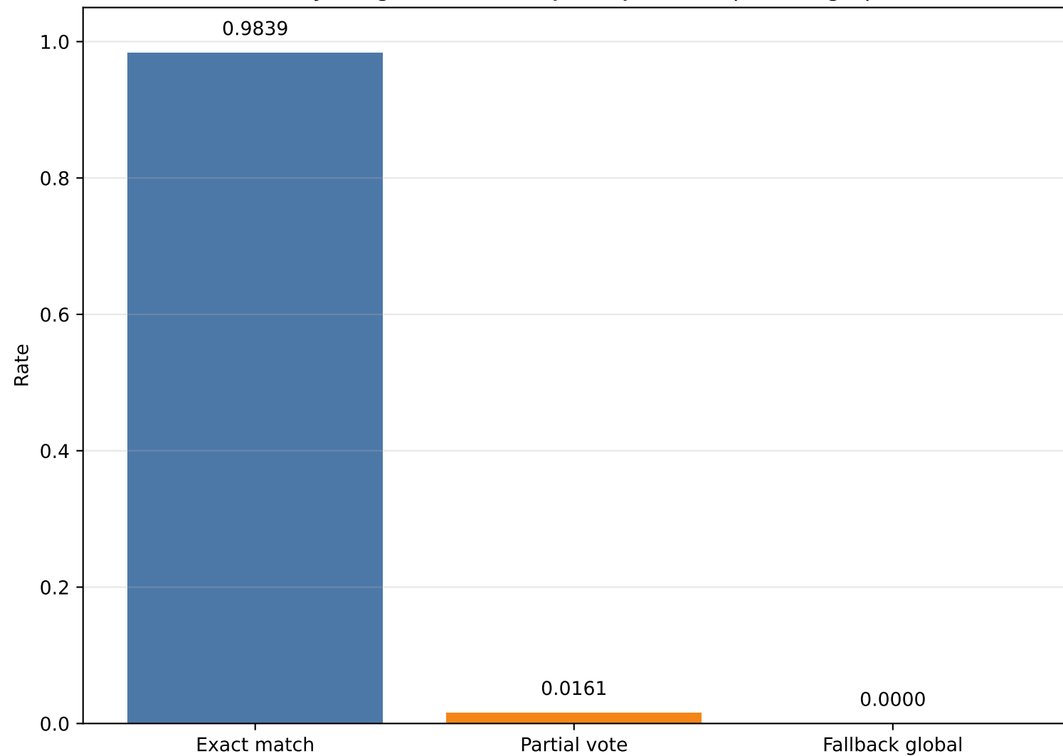
Dictionary Usage Breakdown (JA4 + JA4X complete fingerprints)
