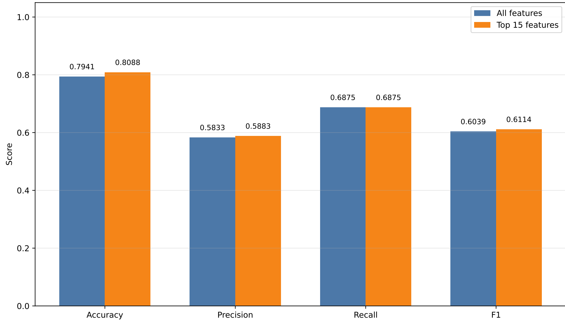
JA4 + JA4S + + JAT + JA4TS features vs Top 15 features - Test Metrics
