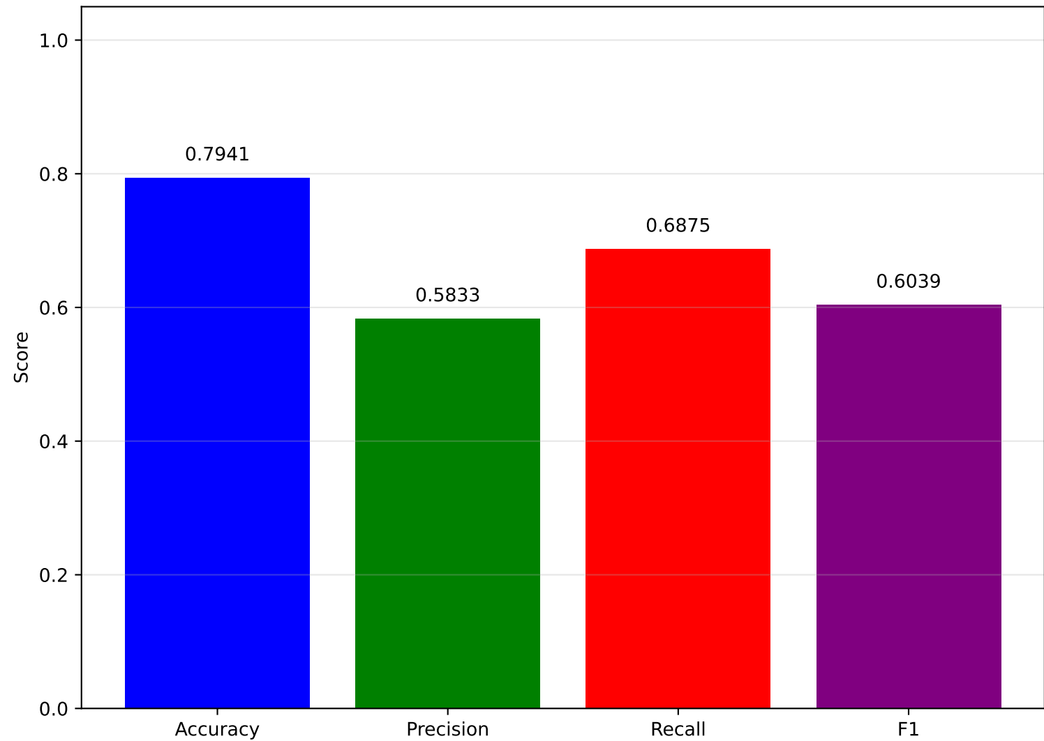
Test Metrics (JA4 + JA4S + JA4T + JA4TS features)
