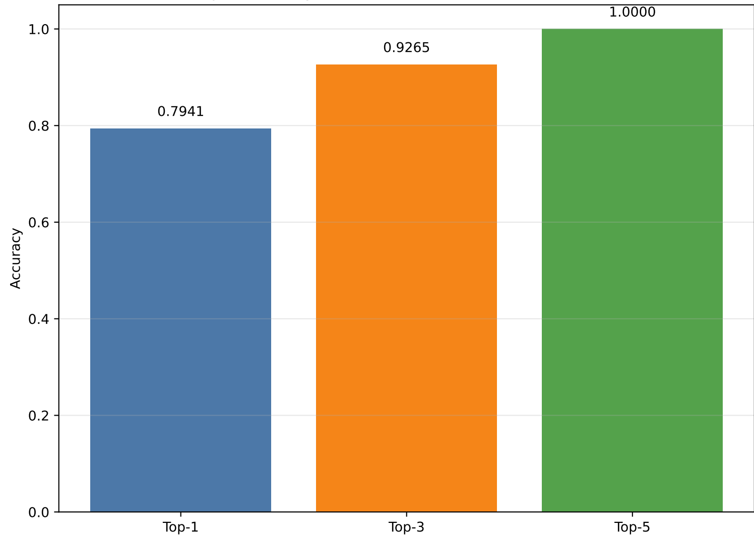
Top-k accuracy (JA4 + JA4S + JA4T + JA4TS features)
