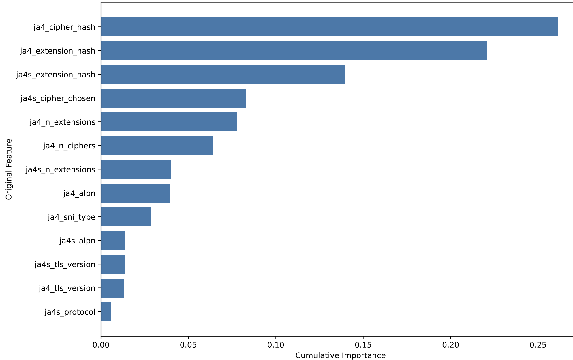
Top 13 Most Important Original Features
