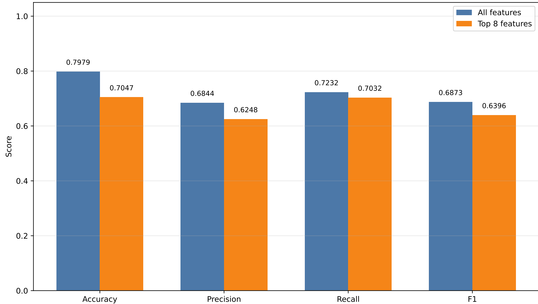
JA4 + JA4S features vs Top 8 features - Test Metrics
