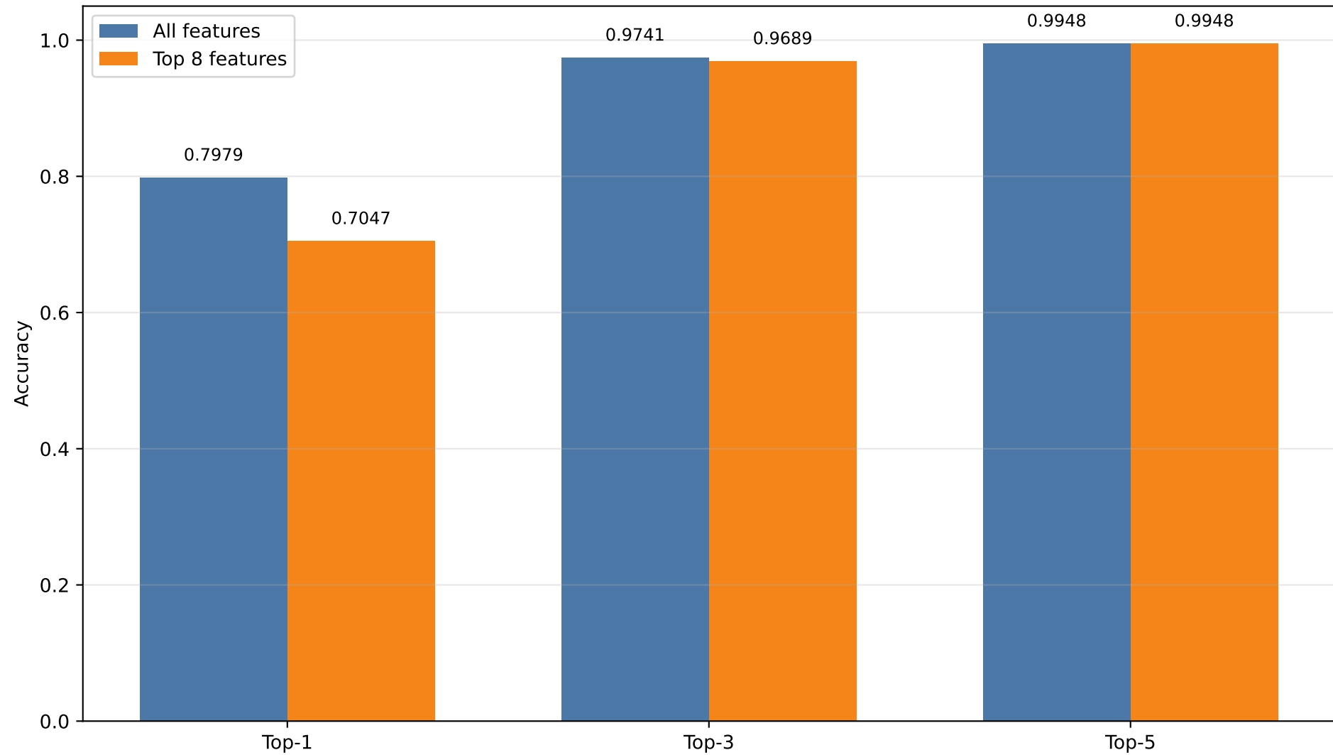
JA4 + JA4S features vs Top 8 features - Top-k accuracy
