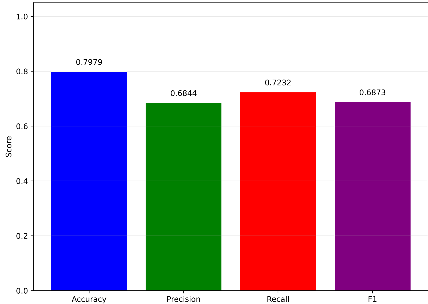
Test Metrics (JA4+JA4S features)
