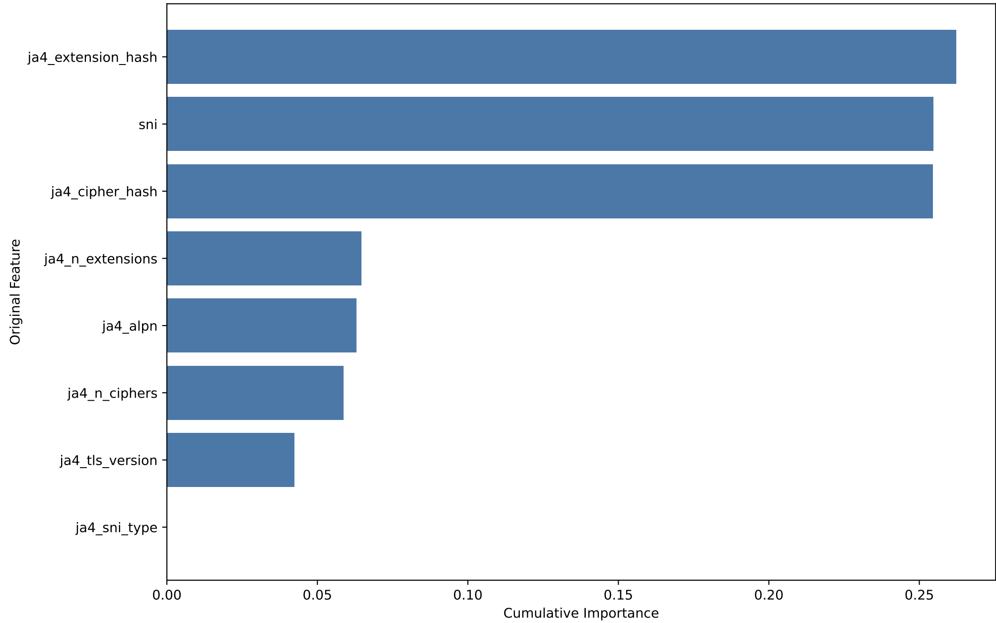
Top 8 Most Important Original Features
